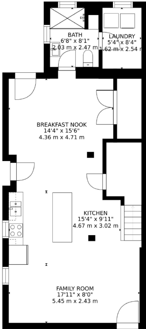
FLOOR 1
